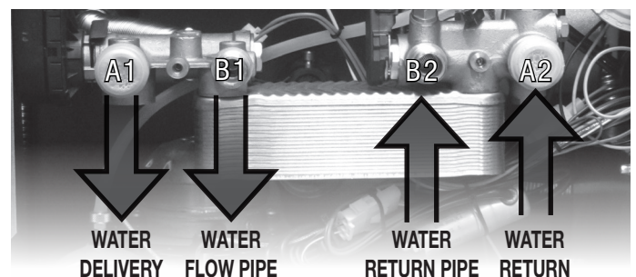
Connection diagram for thermostove equipped with kit for domestic hot water production
